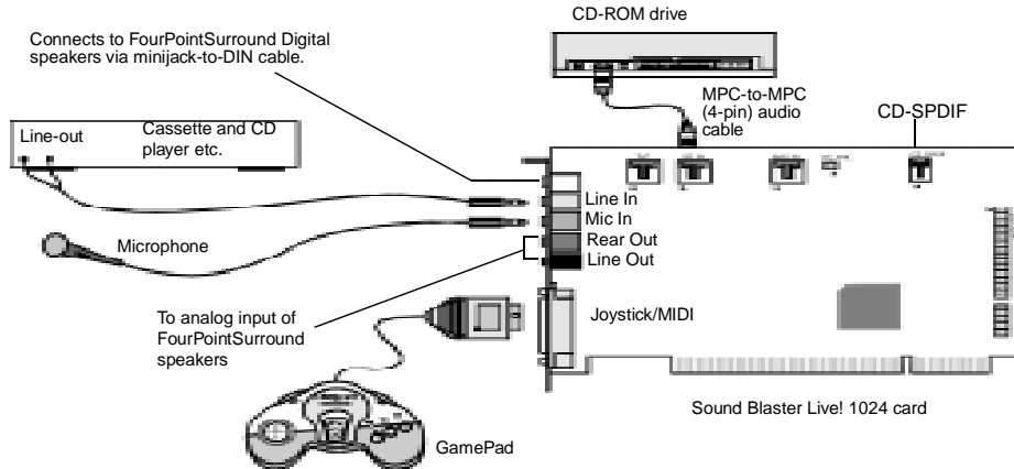
Figure 1-3: Connecting other devices.
